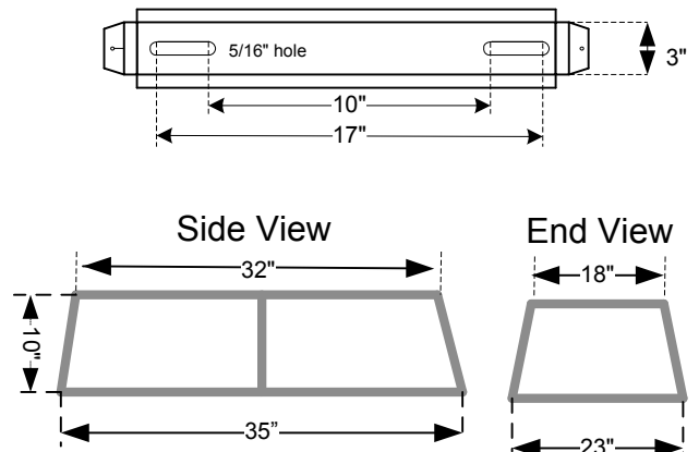
MIN1832 bracket
