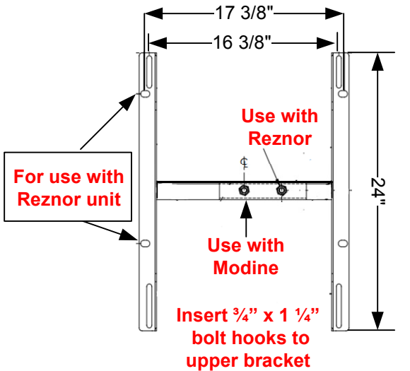
Lower Bracket (bolts to unit) using \frac{3}{4} x \frac{3}{8} " bolts & washers
