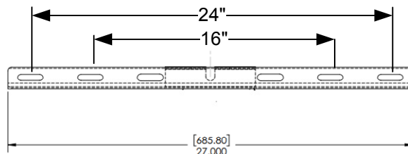
Ceiling Bracket (bolts to ceiling) Using 2 \frac{1}{2} " x \frac{3}{8} " lag bolts & washers
